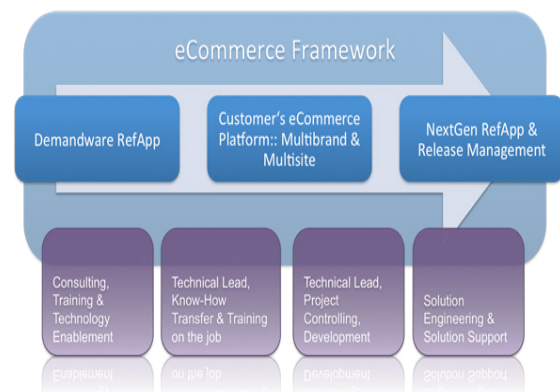
Fig. 2 E-Commerce Framework
