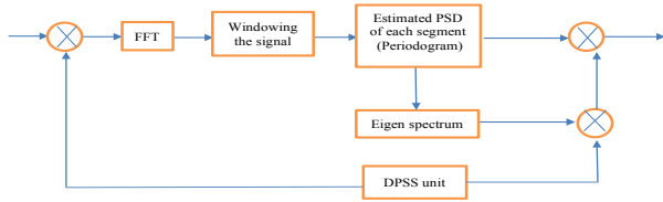
Fig1: Block diagram of multi-taper spectral estimation unit
